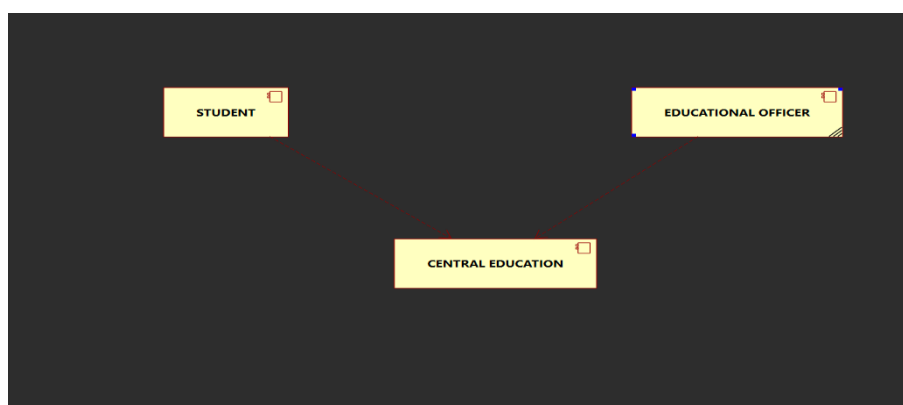
DIAGRAM 7 COMPONENT DIAGRAM
