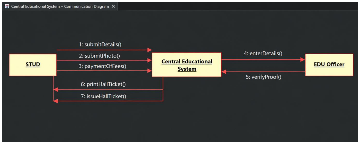
DIAGRAM 4 : COMMUNICATION DIAGRAM
