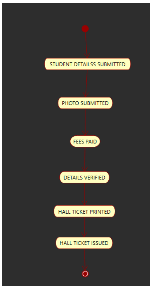
DIAGRAM 5: STATE DIAGRAM
